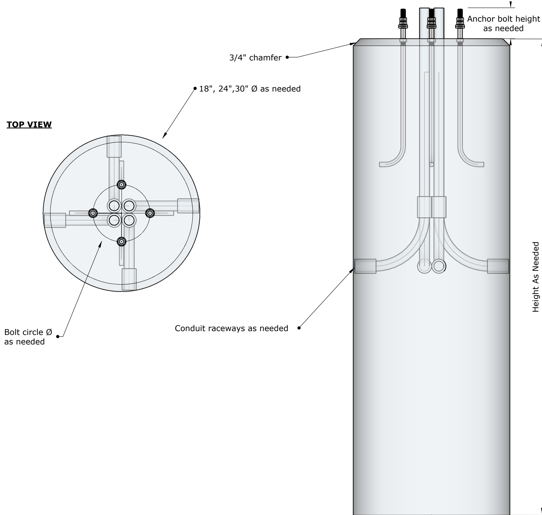
SIDE VIEW
